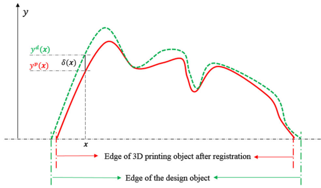
Figure 1. Illustration of dimension deviation of a 3D printing surface, y is the building direction and (x_1, x_2) -plane is the datum reference. \delta(\mathbf{x}) is the dimensional deviation on location \mathbf{x} .
