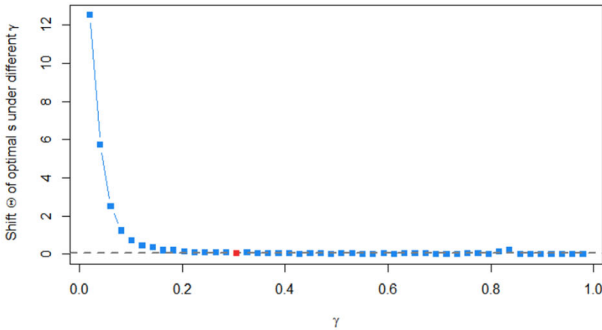
(a) \Theta(k) decreases with \gamma(k) . When \Theta(k) < \theta , the selected \gamma is the red dot. The dashed line indicates the threshold \Theta = \theta .
