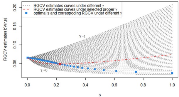
(b) Different RGCV paths versus the value of s ; from top to bottom, the paths are associated with the values of \gamma from 1 to 0; the optimal s , denoted by blue dots, can be found at the lowest point on the RGCV path. Red dashed lines represent the RGCV path with respect to the selected \gamma .
