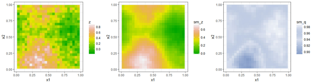
(a) Deformation scheme (i): unsmoothed z (left), z^{(s)} (middle), and scaled quality q (right).
